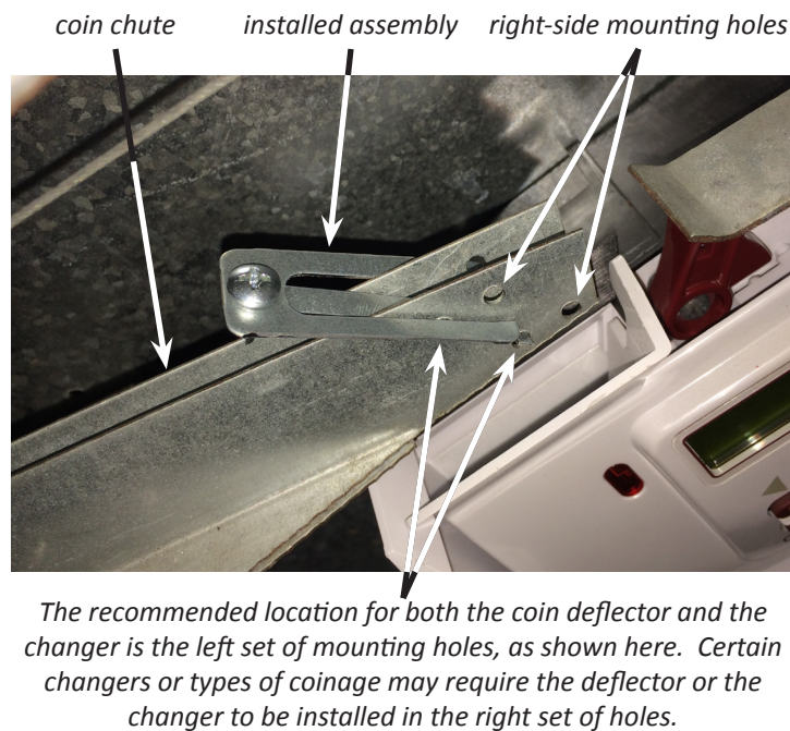
Figure 2. Install the coin deflector assembly on the coin chute as shown here.
