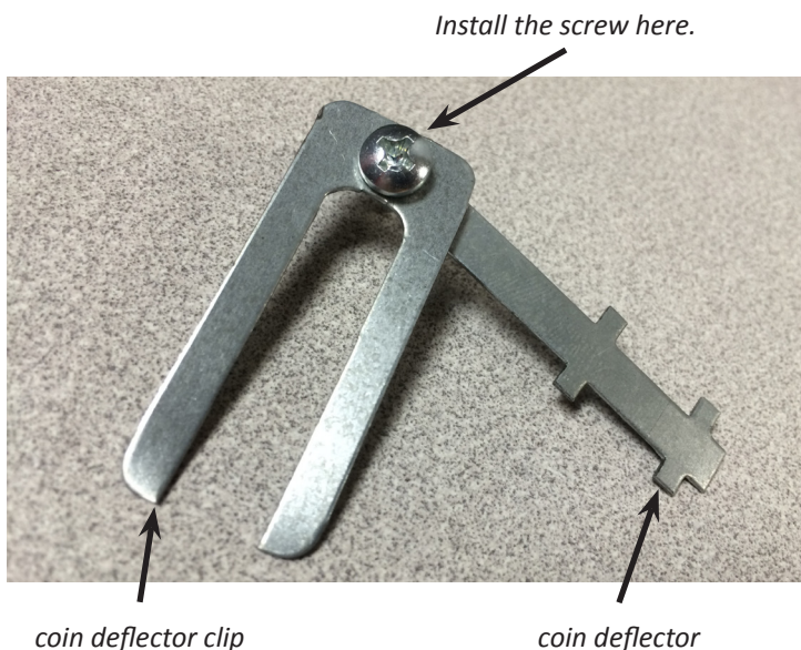
Figure 1. Attach the coin deflector and the clip with the screw, as shown here.
